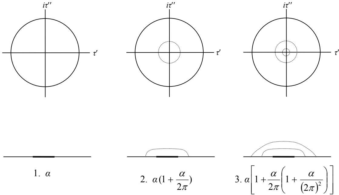
Figure 2; Representation, on the complex time plan, of the self-interaction induced by the QJ.
