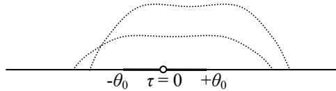
Figure 1; The \theta_0 -neighborhood of a QJ (induced by the action of external fields in \tau = 0 ) is surrounded by k pairs of virtual photons emissions and reabsorption
