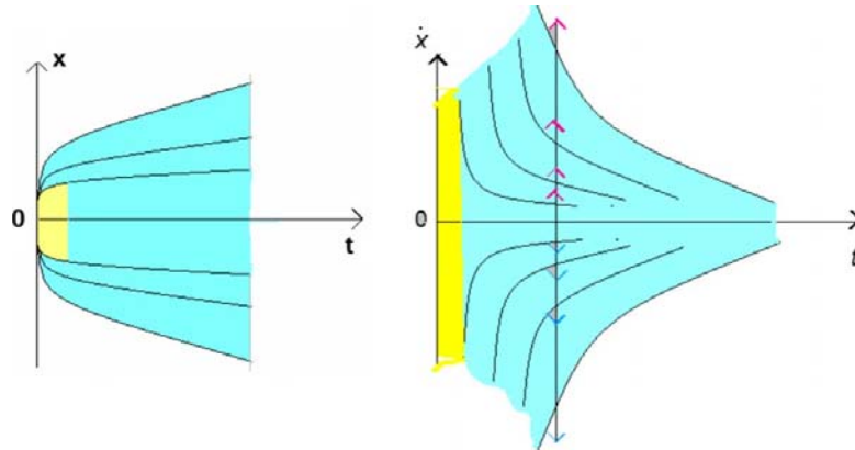
Figure 5. Family of random trajectories and particle velocities
