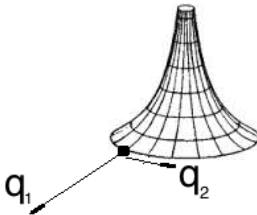
Figure 1. Inertial motion on a smooth pseudosphere
