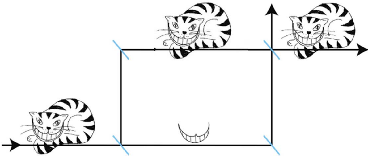
Figure 2 Result of Denkmayr et al. Experiment
