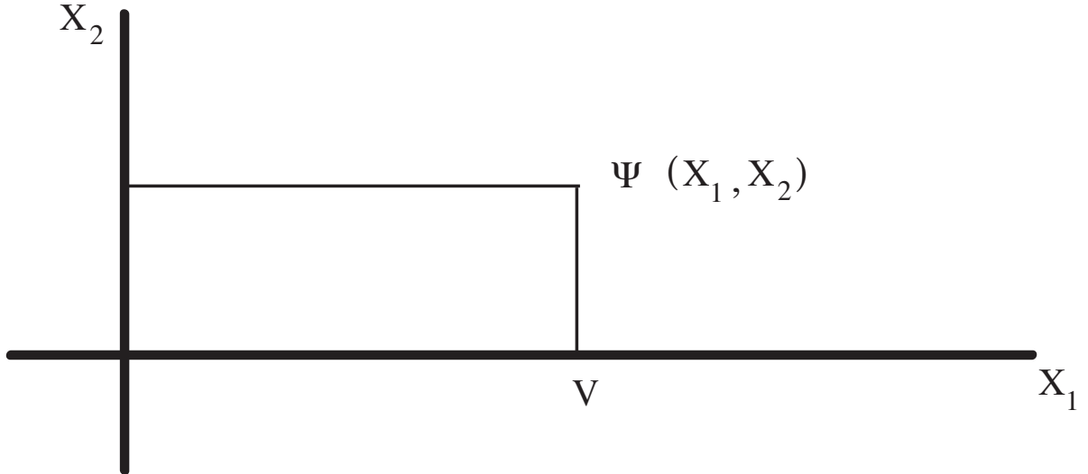
Figure 5: Non locality in de Broglie-Bohm's theory
